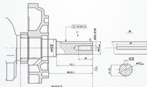
186F/188F/192F Keyway Shaft
